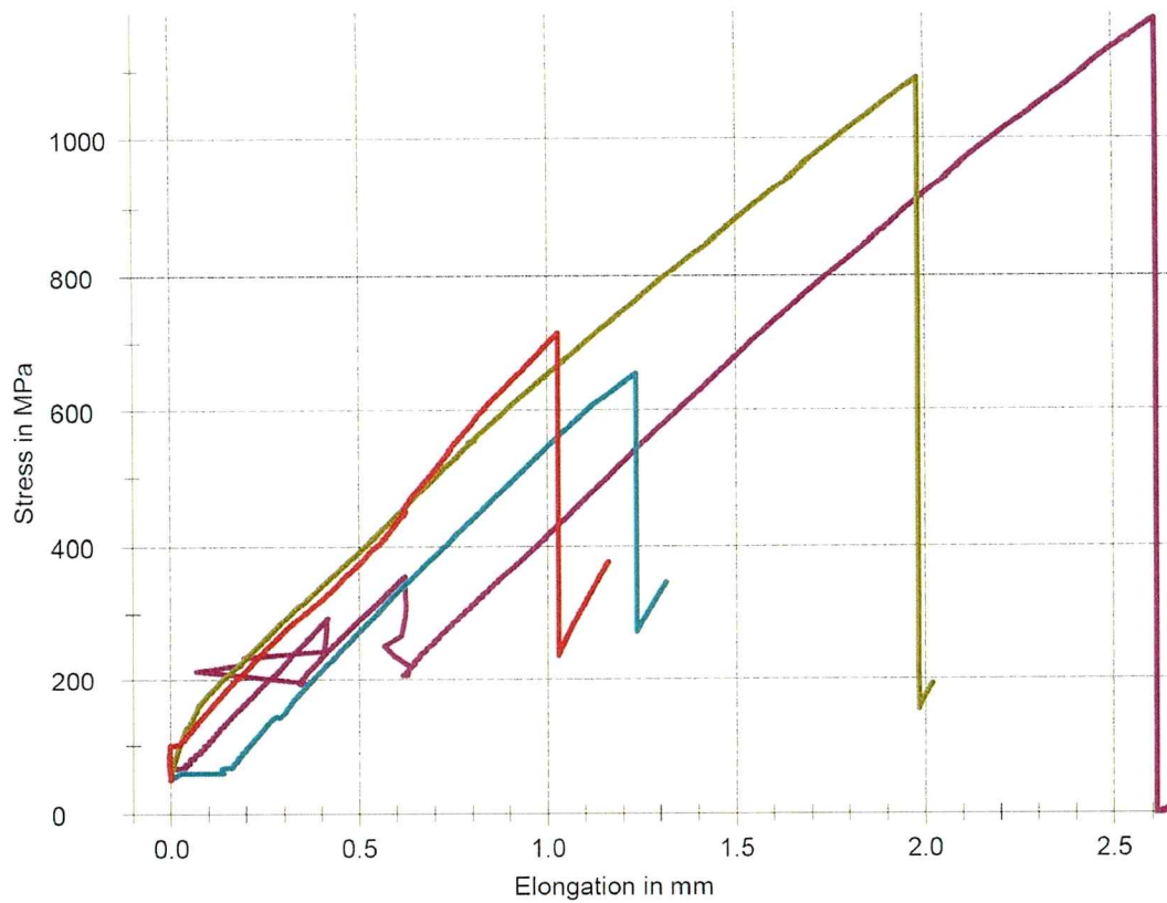
Fig. 2.. Results of the tension tests for 12 mm diameter samples.
