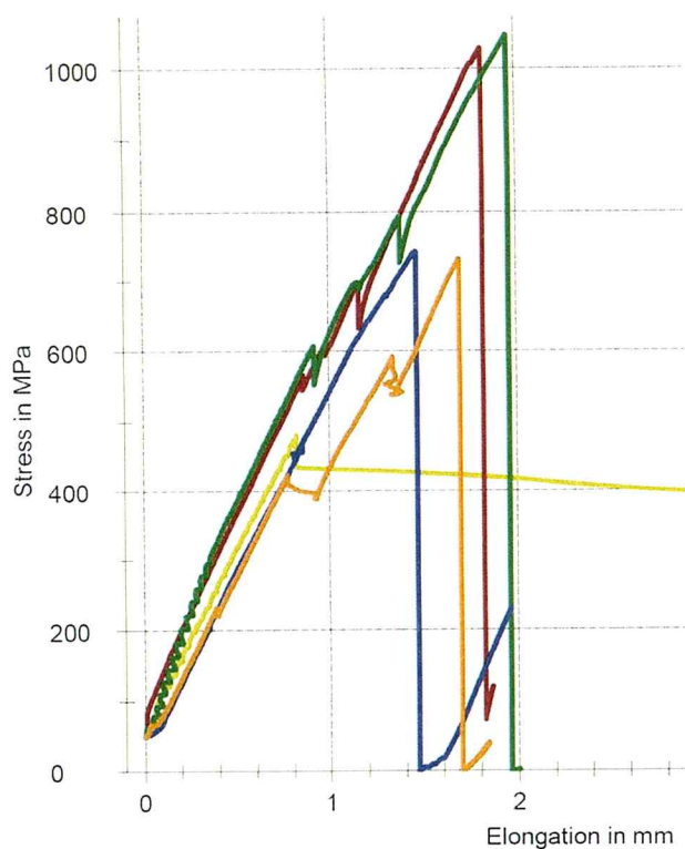
Fig. 2.. Results of the tension tests for 10 mm diameter samples.
